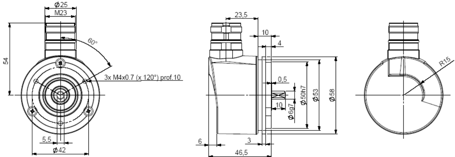
CHM5_06 connection CPR / C1R (radial M23), with flange 9500/003 mounted on the body
